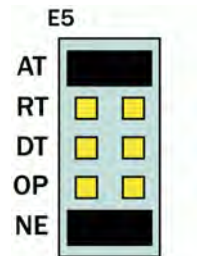
Figure 2 - Header E5, RS-485 'Auto' Enabled, with 'No Echo'
