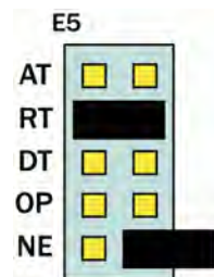
Figure 5 - Header E5, RS-485 'RTS' Enabled, with 'Echo'
