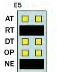
Figure 4 - Header E5, RS-485 'RTS' Enabled, with 'No Echo'
