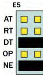
Figure 6 – Header E5, RS-485 ‘DTR’ Enabled, with No Echo
